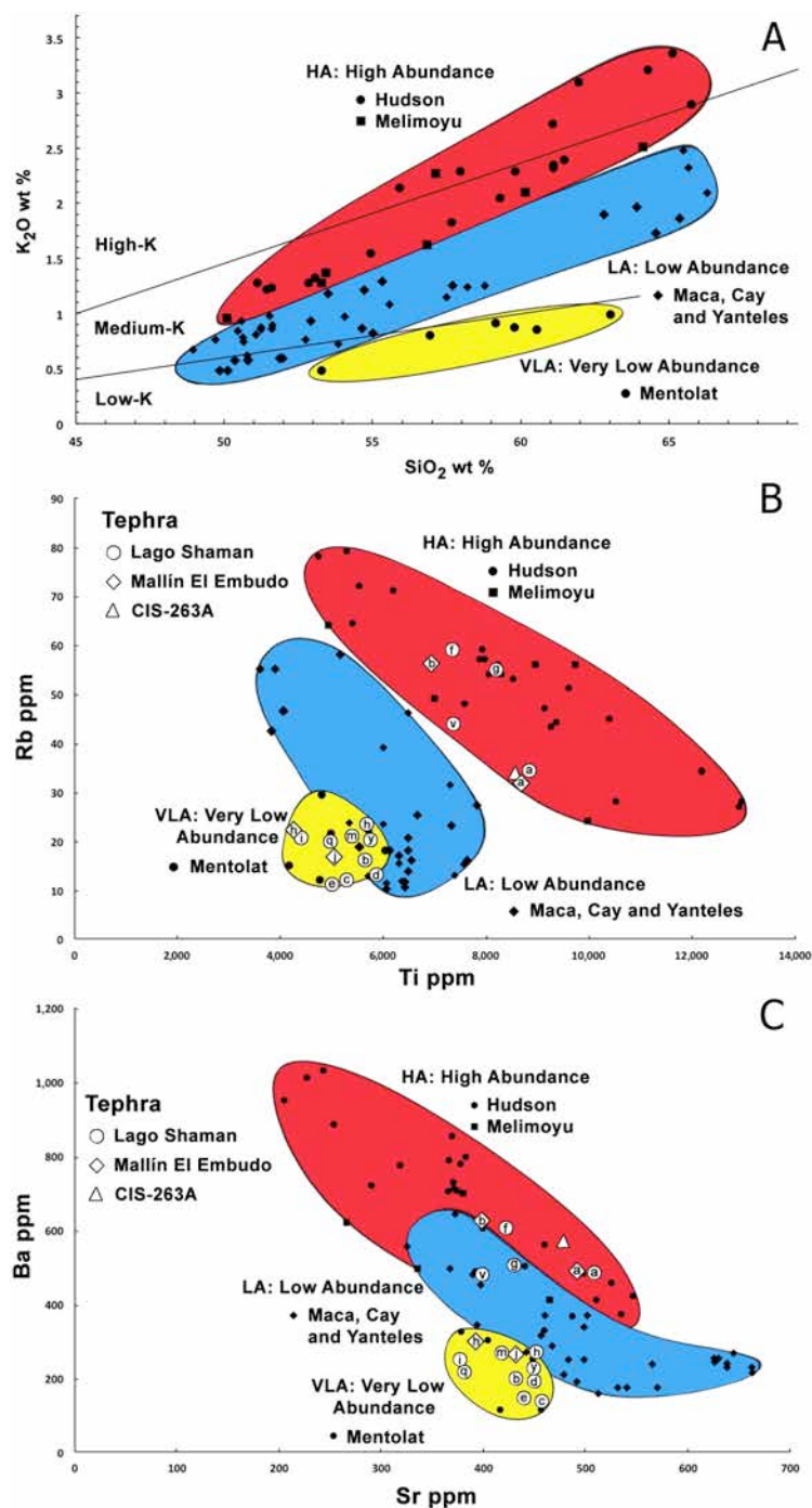
FIG. 6. A. SiO 2 versus K 2 O for samples of both lavas and tephra from Yanteles, Melimoyu, Maca, Cay and Hudson volcanoes (Futa and Stern, 1988; López-Escobar et al. , 1993; Naranjo and Stern, 1998, 2004; D’Orazio et al. , 2003; Gutiérrez et al. , 2005; Kratzmann et al. , 2009, 2010), illustrating the separation of these samples into what have previously been termed High, Low and Very Low Abundance magma types (Hickey et al. , 1986, 1989, 2003; López-Escobar et al. , 1993, 1995a, 1995b; Sellés et al. , 2004; Watt et al. , 2011). Line separating the fields of High-, Medium-, and Low-K convergent plate boundary magmas are from Peccerillo and Taylor (1976); B. Ti versus Rb for the SSVZ volcanoes and each individual tephra from the upper Río Cisnes valley (Table 3); C. Sr versus Ba for the SSVZ volcanoes and tephra from the upper Río Cisnes valley (Table 3).
